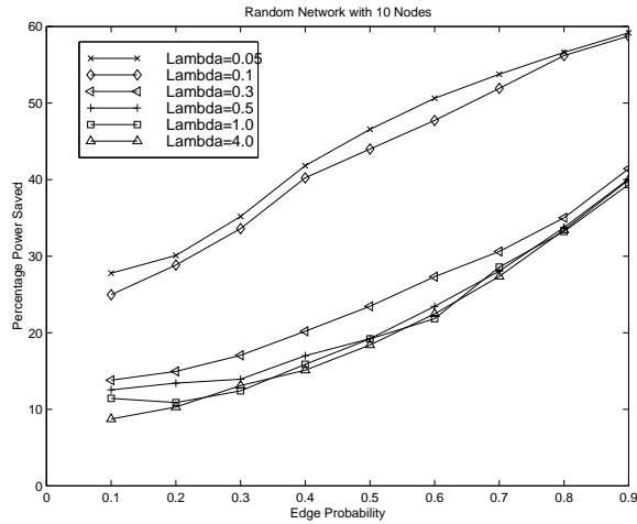
Figure 9: Power saved in random networks with 10 nodes.
