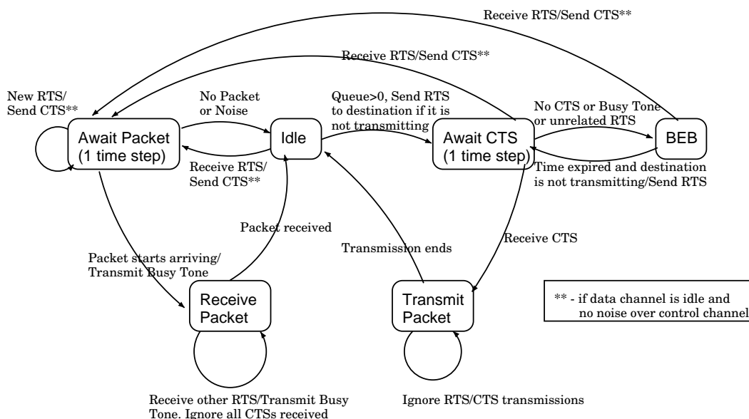
Figure 4: The PAMAS Protocol.
