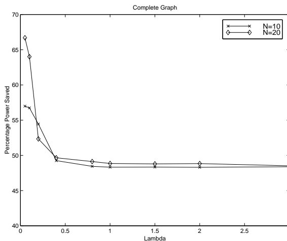
Figure 7: Power saved in complete networks with 10 or 20 nodes.
