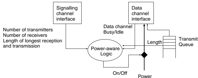
Figure 6: Separate interfaces for signalling and data.
